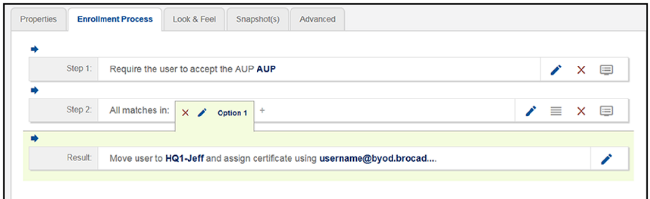
FIGURE 25 Workflow Before Adding DPSK Branch
